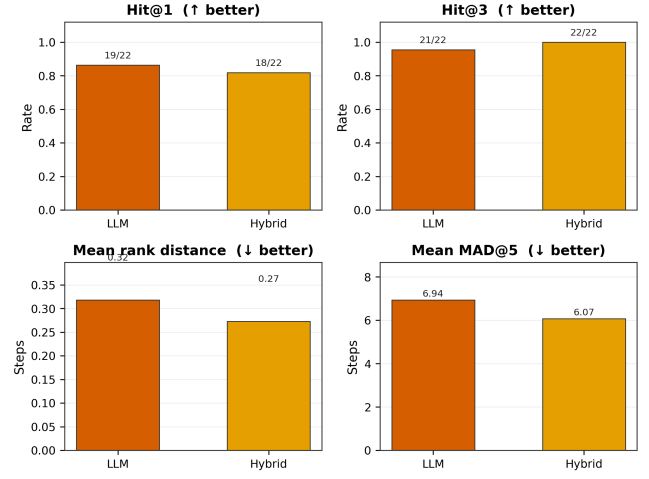
v2 — LLM vs Hybrid: complementary metrics (22 traces)
