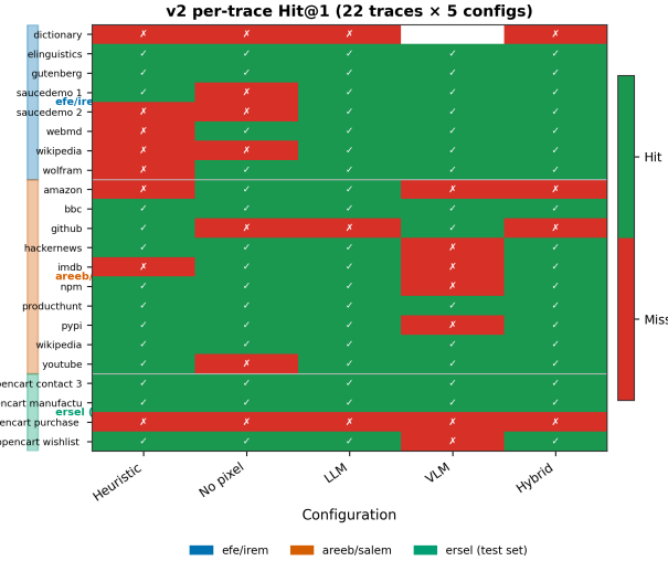
Figure 6: Per-trace Hit@1 heatmap (v2). Left band: source collection (ersel = test set).
