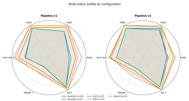
Figure 5: Multi-metric radar comparison across v1 and v2 modes (Hit@1/3/5, rank distance, MAD@5).
