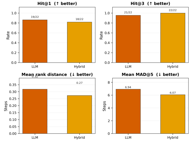
v2 — LLM vs Hybrid: complementary metrics (22 traces)
