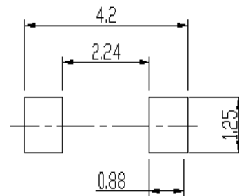
Soldering footprint
