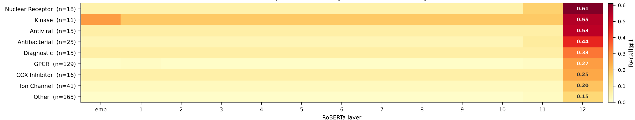
(A) Per-mechanism-family Recall@1 across RoBERTa layers (text\_rich) All families peak at the final layer; value annotated at layer 12.
