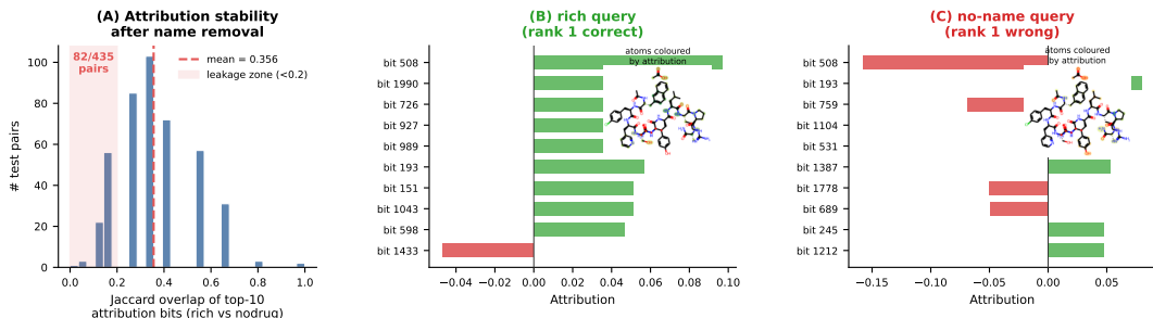
Figure 5: Drug-name leakage changes the substructures used by the same model. The rich query includes the explicit drug name, while the no-name query removes only that span at inference with all model weights fixed. Low top-10 ECFP4 saliency overlap means that removing lexical information changes which molecular environments drive retrieval. Cetorelix acetate illustrates a leakage candidate where the prediction and salient substructures both shift after the name is removed.
