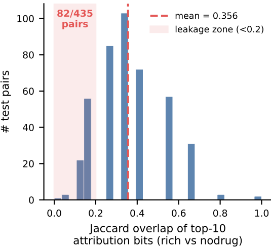
(A) Attribution stability after name removal
