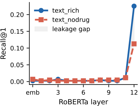
(A) Recall@1
