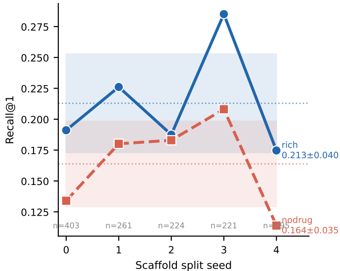
(B) Multi-seed stability 5 independent scaffold splits
