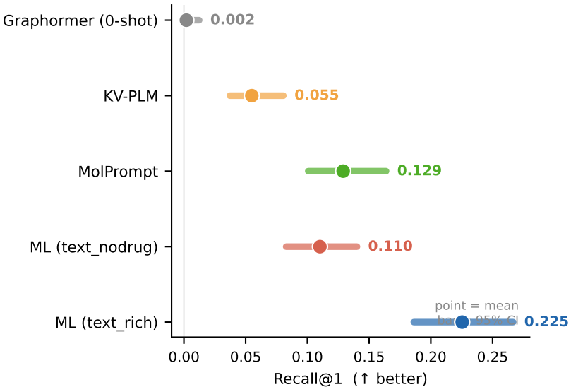
(A) Bootstrap 95% CI Recall@1 — N = 435 test pairs
