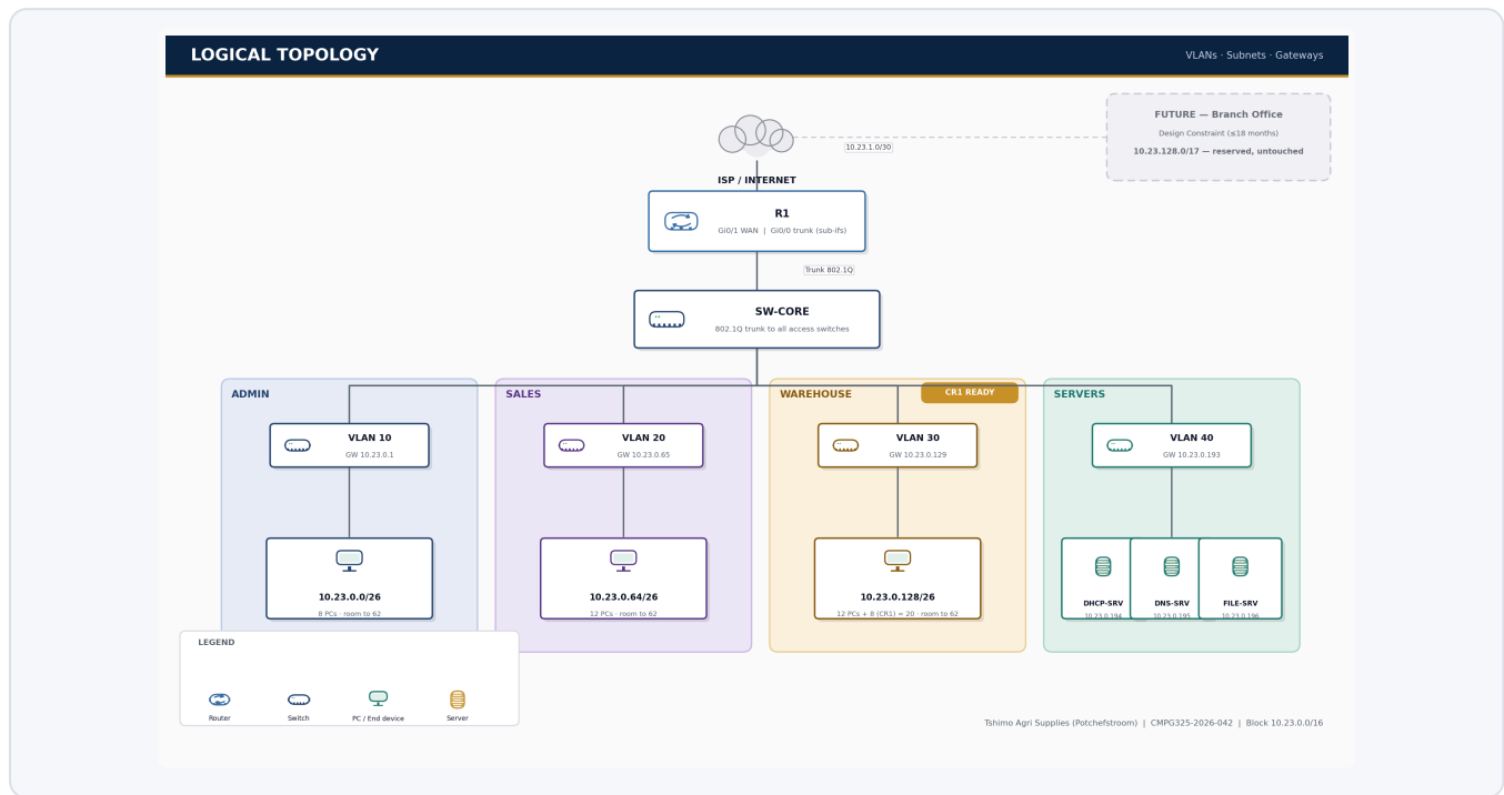
Figure 2 — Logical Topology: VLANs, subnets and default gateways
