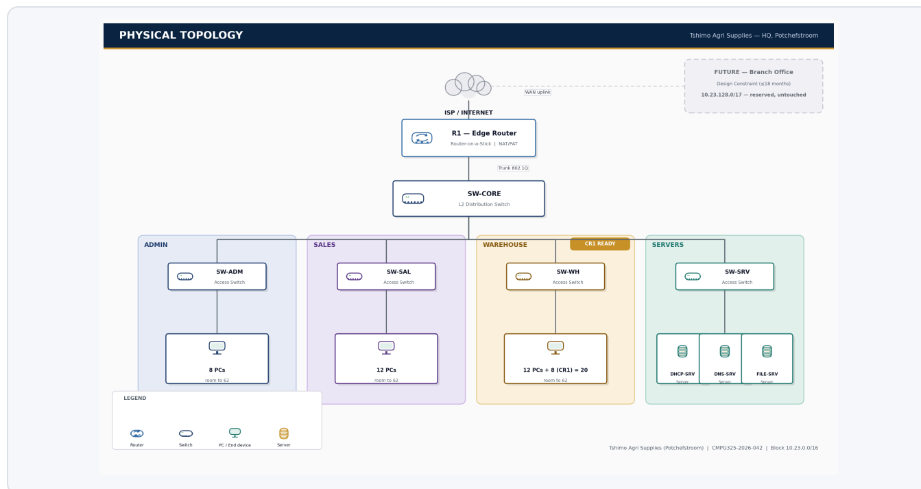
Figure 1 — Physical Topology, Tshimo Agri Supplies HQ (Potchefstroom)
