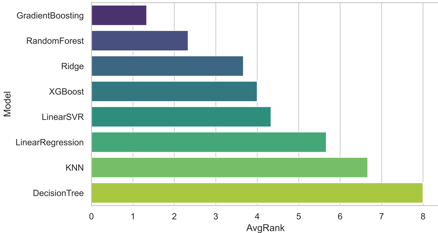
RQ5 — Average rank across MAE, RMSE, R^2 (lower is better)
