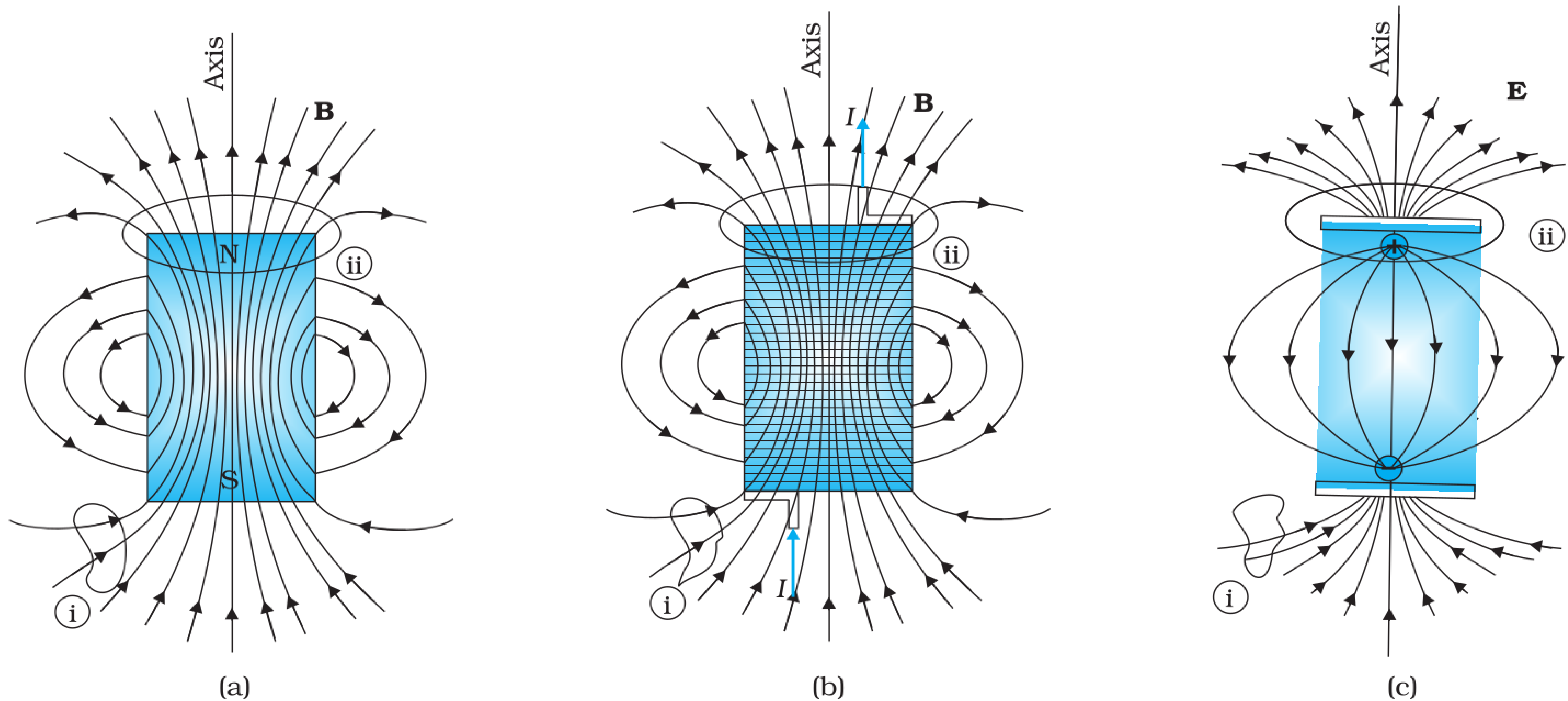
FIGURE 5.3 The field lines of (a) a bar magnet, (b) a current-carrying finite solenoid and (c) electric dipole. At large distances, the field lines are very similar. The curves labelled (i) and (ii) are closed Gaussian surfaces.
