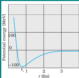
FIGURE 13.2 Potential energy of a pair of nucleons as a function of their separation.
