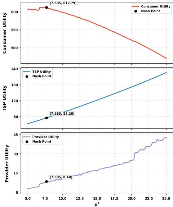
Vary service consumer strategy (exp_eta_scale_2_5)
