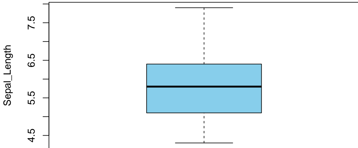
Box plot for Sepal Length
