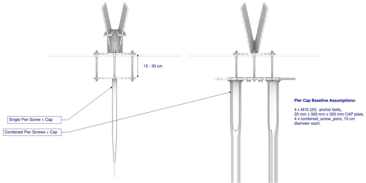
Section_View
