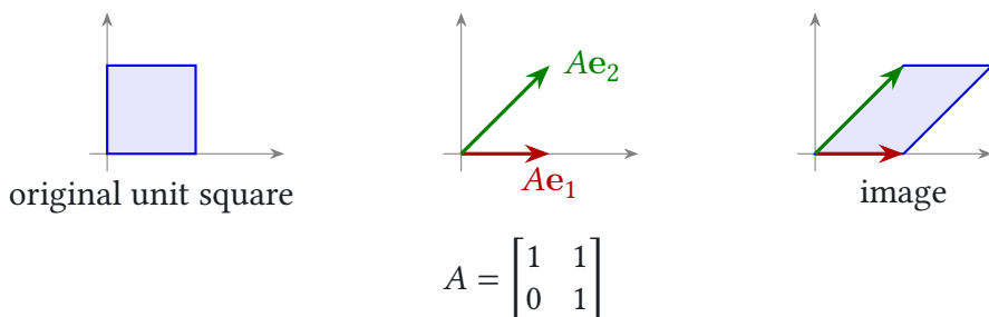
Figure 1.7. A 2 \times 2 matrix sends the unit square to the parallelogram determined by its two columns. This is the geometric version of columns contribute.
