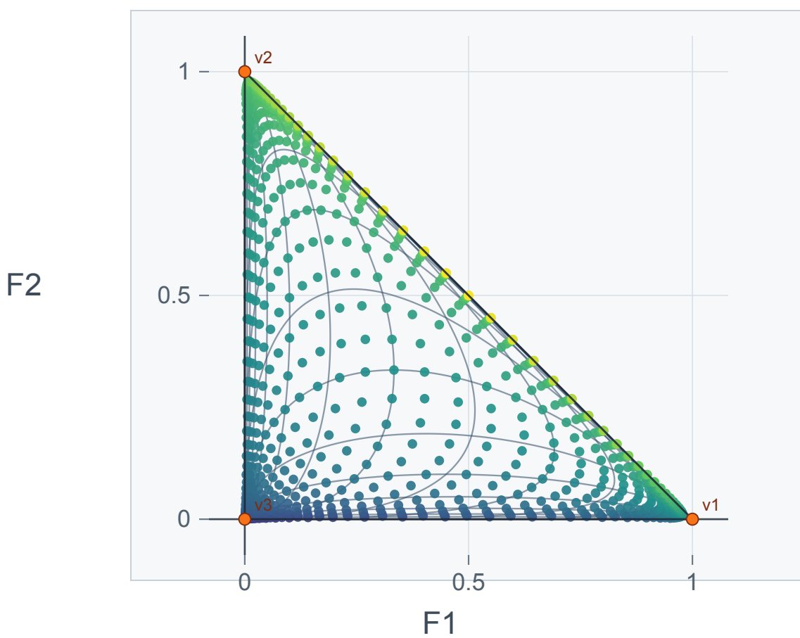
Softmax-weighted image
