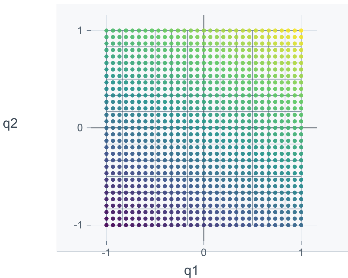
Query grid
