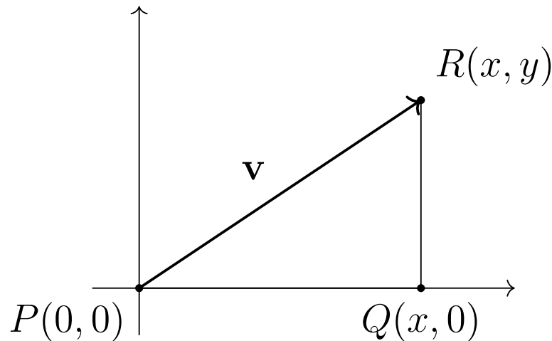
Figure. A triangle with vertices P(0, 0) , Q(x, 0) , and R(x, y) , drawn to determine the length of the line-segment upon which a 2-vector is based.
