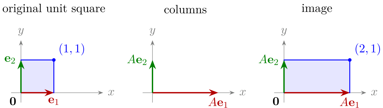
Figure. A 2 \times 2 matrix sends the unit square to the parallelogram determined by its two columns. This is the geometric version of columns contribute.
