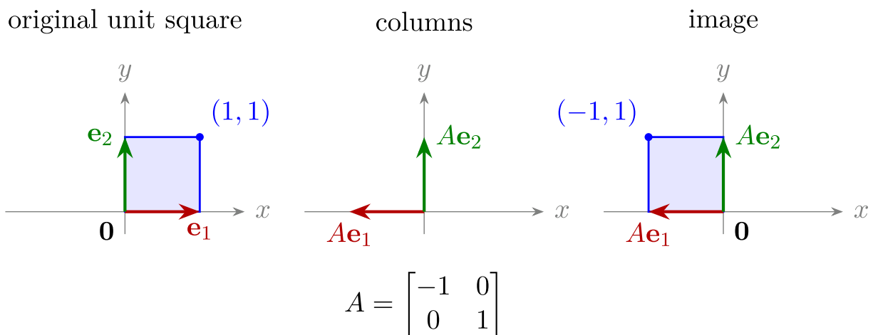
Figure. Reflection across the y -axis sends the unit square to its left-hand mirror image. The first column reverses the horizontal direction, while the second column leaves the vertical direction unchanged.
