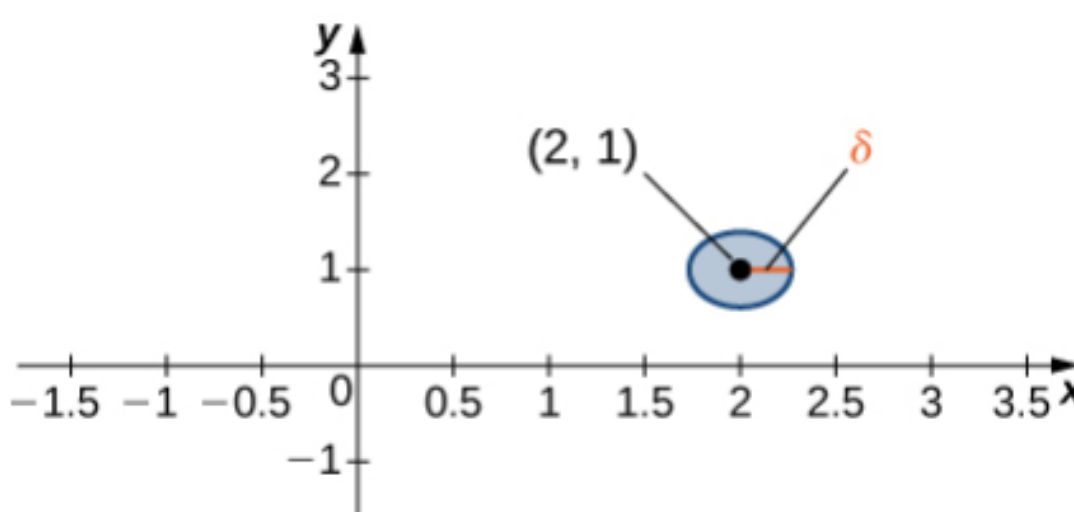
Figure. A \delta -disk centered around the point (2, 1) . Figure 4.14 from Edwin “Jed” Herman and Gilbert Strang, Calculus Volume 3 , OpenStax, © 2018 Rice University, licensed under CC BY-NC-SA 4.0; source: OpenStax Figure 4.14 .
