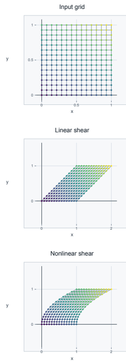
Figure. Square-grid visualization for T(x, y) = (x + y, y) and F(x, y) = (x + y^2, y) . The color identifies the original input point. The two maps agree on the four corners, but the nonlinear map bends grid lines.
