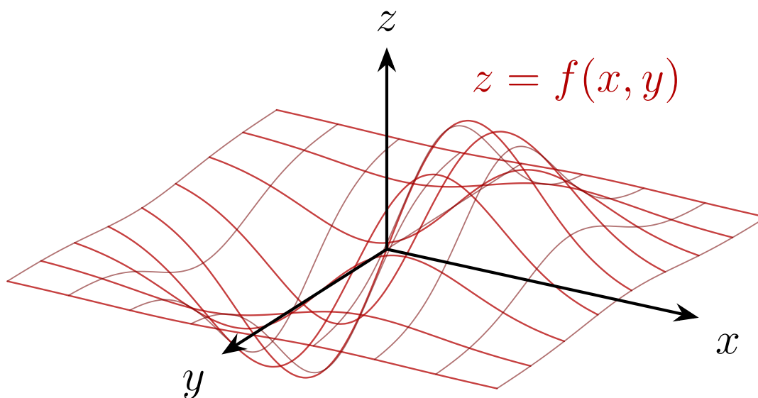
Figure. A graph of the function f(x, y) = xe^{-x^2-y^2} .
