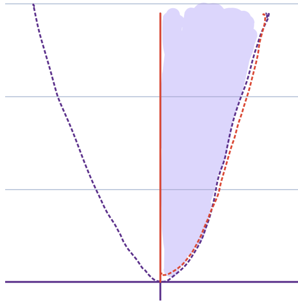
Figure. Domain of f(x, y) = \ln(y - x^2) + \sqrt{x} . Figure by Melissa Lindsey.
