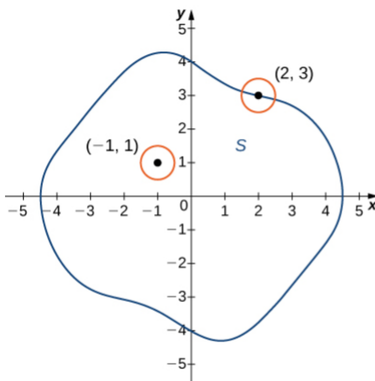
Figure. A planar set with one interior point and one boundary point marked.
