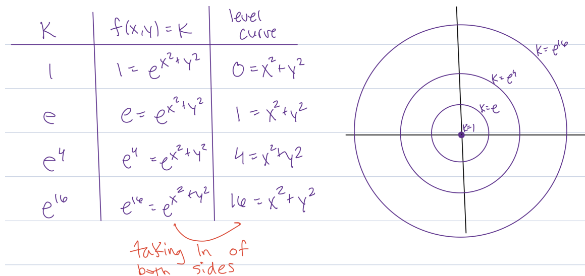
Figure. Level curves of f(x, y) = e^{x^2+y^2} . Figure by Melissa Lindsey.
