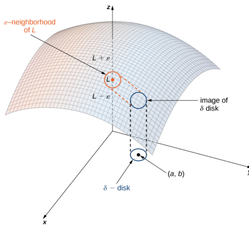
Figure. Epsilon-delta diagram for a two-variable limit on a surface.
