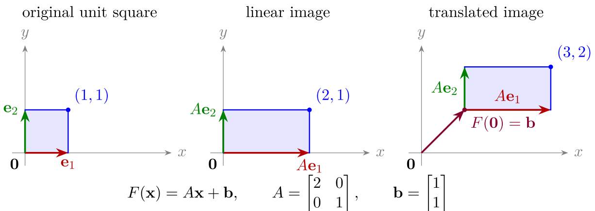
Figure. A unit square is stretched horizontally and then translated one unit right and one unit up.
