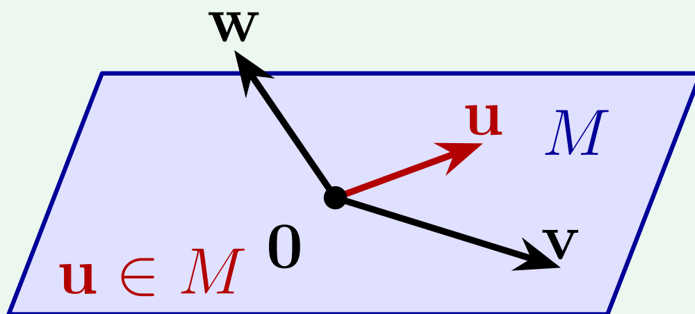
Figure. \{u, v, w\} dependent.
