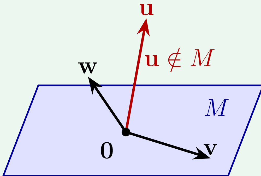
Figure. \{u, v, w\} independent.
