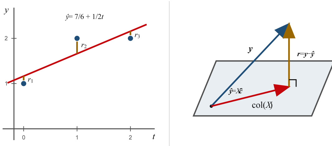
Figure 4.3. Two views of the same line fit. In the data plot, the residuals are vertical differences r_i = y_i - \hat{y}_i . In \mathbb{R}^3 , the fitted vector \hat{\mathbf{y}} = X\hat{\mathbf{c}} is the projection of \mathbf{y} onto \text{col}(X) , and \mathbf{r} \perp \text{col}(X) .
