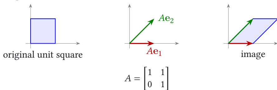
Figure 1.9. A 2 \times 2 matrix sends the unit square to the parallelogram determined by its two columns. This is the geometric version of columns contribute.
