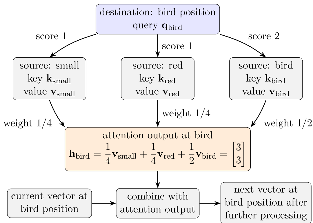
Figure. Attention at the bird position combines value vectors from small, red, and bird.
