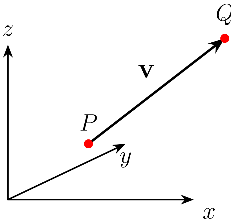
Figure. A vector \mathbf{v} represented as an arrow between two points P and Q .
