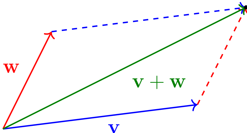
Figure. The sum of two vectors \mathbf{v} and \mathbf{w} .
