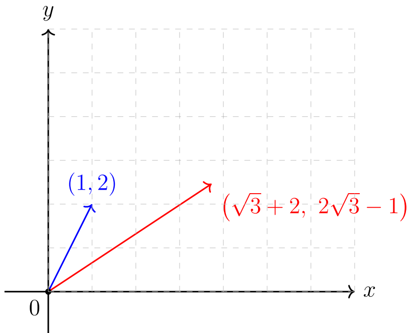
Figure. The vectors \mathbf{v} and \mathbf{w} from the activity, drawn as arrows from the origin.
