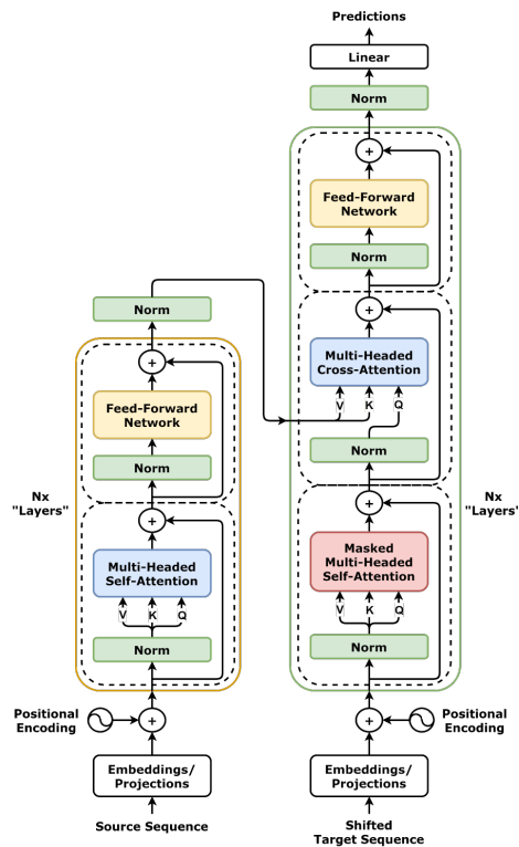
Figure. A transformer processes a sequence of token vectors. The activities below focus on the vector operations visible in the diagram: token embeddings, dot-product scores, weighted averages, and affine layers. Source: Wikipedia, Transformer (deep learning architecture), using Transformer, full architecture.png by dvigodoy, licensed under CC BY 4.0.
