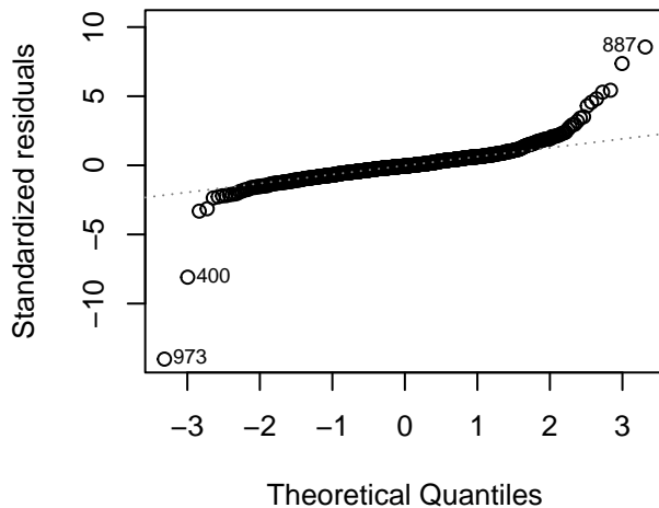
Q-Q Residuals
