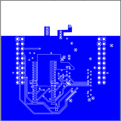
GND (Scale 1:1)
