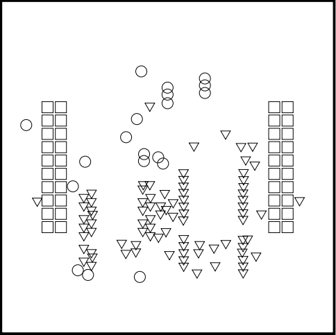
Drill Drawing View (Scale 1:1)
