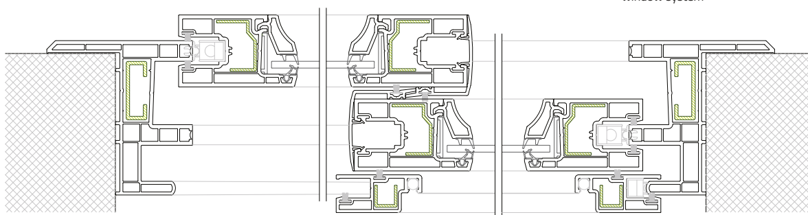
Section C Horizontal section of complete window system
