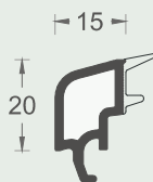
EMA4278 Double glazing bead 25 pieces/ package
