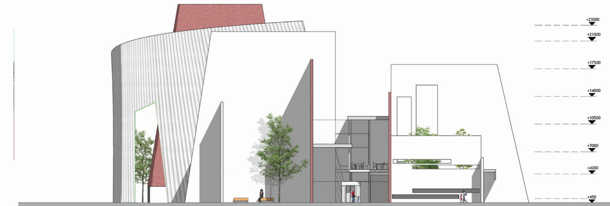
SOUTH ELEVATION 1/250
