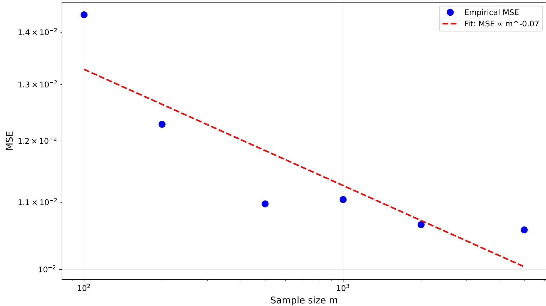
Convergence Rate: Empirical -0.07 vs Theoretical -0.67
