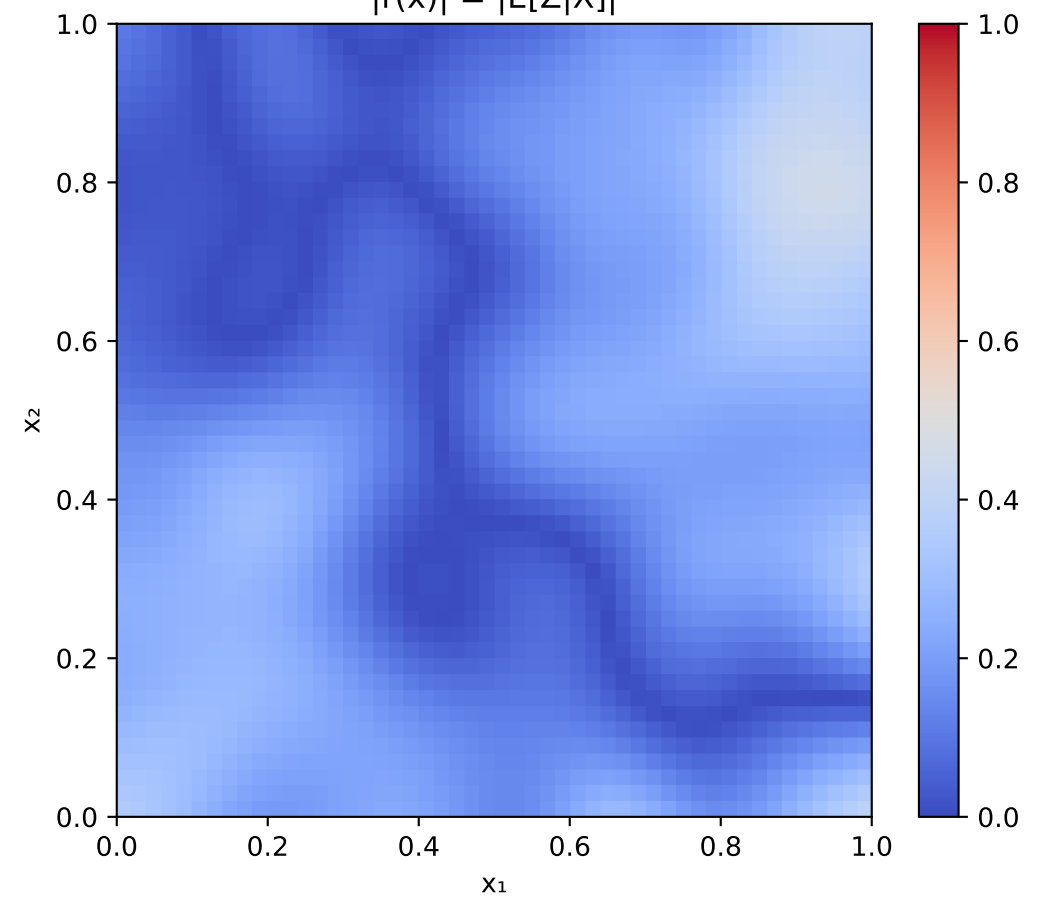
|\hat{r}(x)| = |E[Z|X]|
