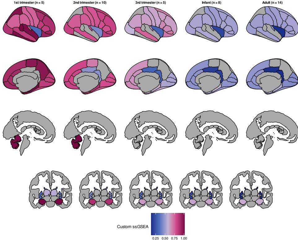
Fig. 4 User-submitted gene-list mode. ssGSEA computed on demand for the dorsal/glutamatergic specification programme that ? report as upregulated by chronic intermittent ethanol exposure in human pluripotent stem cells differentiated to first-trimester-equivalent cortical neurons ( EMX2 , LHX1/2/5/9 , OTX2 , FEZF2 , NEUROD1/2/6 , NEUROG2 , TBR1 , EOMES ). The submitted list is a published differential-expression result, not a curated marker panel, and it is mapped without local installation or coding. The score is highest in the cortical parcels of the first two prenatal windows—the period the in vitro model corresponds to—and falls monotonically thereafter, while the striatum stays low throughout, recovering the dorsal–ventral contrast the signature encodes.
