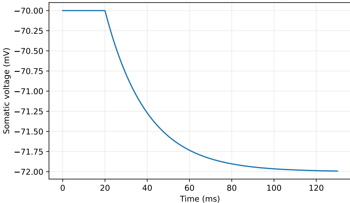
Standard passive current step — SYN1_P10
