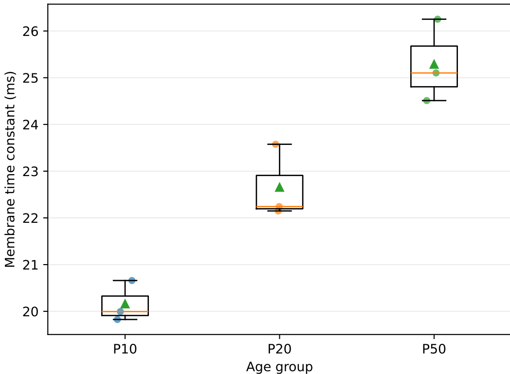
Membrane time constant (ms) across reconstructed OPCs
