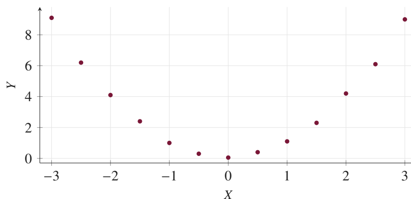
Figure 4.1: Schematic nonlinear relationship: a strong pattern can coexist with approximately zero linear correlation. Coordinates are illustrative.
