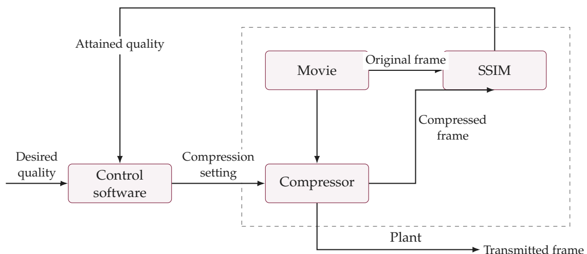
Figure 2.1: Detailed plant boundary from source p. 4. Both original and compressed frames reach SSIM; attained quality returns to the controller.
