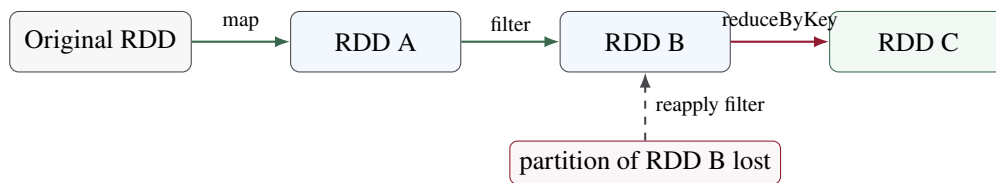
Figure 3.6: Lineage-based recovery. If a partition of RDD B is lost and the required RDD A partition still exists, Spark re-applies the recorded filter only for the missing partition.
