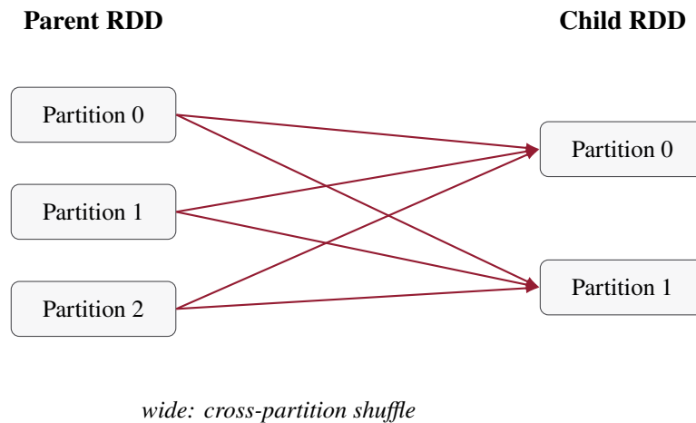
Figure 3.5: Wide dependency: each child partition may require records originating from several parent partitions, forcing network redistribution.
