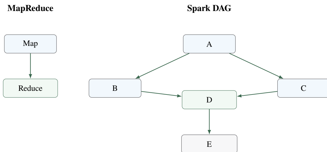
Figure 3.1: A fixed MapReduce pipeline compared with an arbitrary Spark computation DAG. Spark can represent branches, joins, and deeper operation chains rather than exactly one Map and one Reduce phase.
