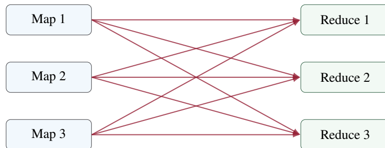
Figure 2.2: The all-to-all structure of shuffle. Every Map task may contribute data to every Reduce task.
