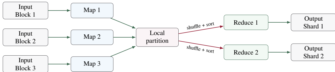
Figure 2.1: MapReduce execution overview: input blocks generate Map tasks; intermediate data is partitioned, shuffled, sorted, and reduced into output shards.
