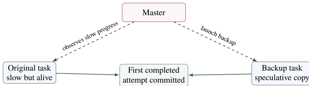
Figure 2.3: Speculative execution: the runtime duplicates a slow task and accepts the first successful attempt.
