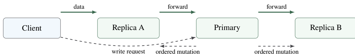
Figure 1.6: GFS write control and data flow. Data is pipelined through replicas, while mutation ordering is controlled by the lease-holding primary.
