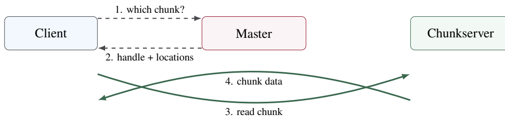
Figure 1.5: GFS read path. The Master supplies metadata; bulk data bypasses the Master and flows directly between the client and a Chunkserver.
