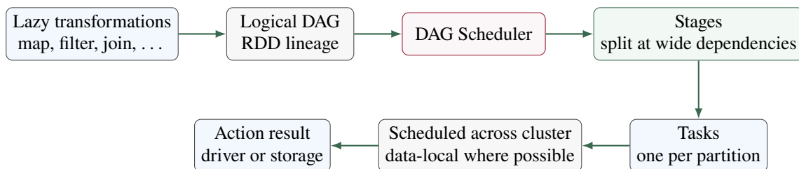
Figure 3.7: Spark execution model from lazy transformations to physical tasks. Narrow chains are pipelined within stages, while wide dependencies introduce shuffle boundaries between stages.
