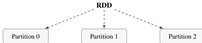
Figure 3.2: An RDD is logically one dataset but is physically processed as independent partitions distributed across the cluster.
