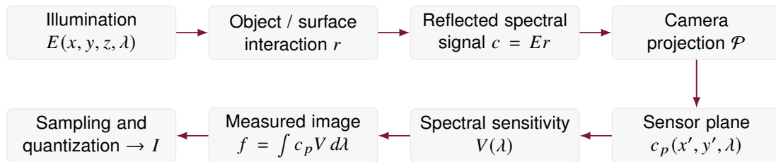
Figure 8.1. Acquisition chain connecting the lecture’s physical, geometric, spectral, and digital stages. Symbols are defined in the following equations; I is the digital image.
