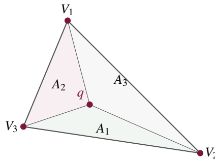
Figure 10.3. Triangle construction: A_i is the sub-triangle opposite vertex V_i . Normalize by A_1 + A_2 + A_3 to obtain area weights.
