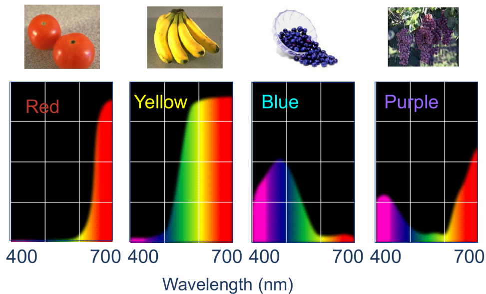
Figure 11.2. Representative surface reflectance spectra shown in the lecture for red, yellow, blue, and purple surfaces.
