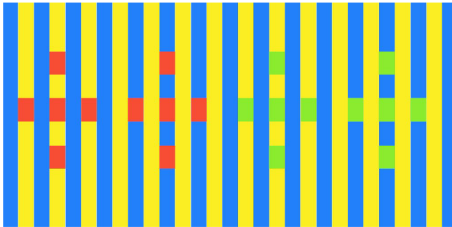
Figure 13.1. The source’s simultaneous-contrast/Mach-band demonstration. The colored targets are viewed within alternating surrounding stripes; the perceptual artwork is preserved.
