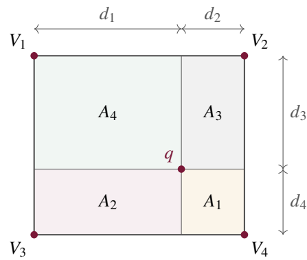
Figure 10.4. Bilinear geometry redrawn from the source: d_1 + d_2 = d_3 + d_4 = 1 in the unit cell. Each corner uses the opposite rectangle's area; Q is the value at q . The drawing is enlarged for readability.
