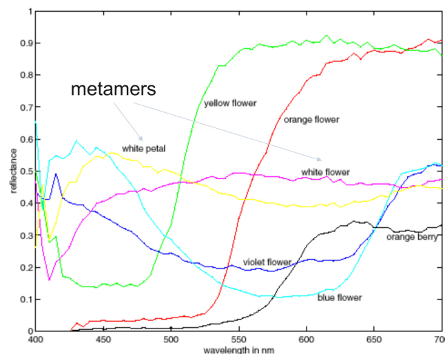
Figure 11.5. Real-world spectral curves used in the lecture to illustrate that different spectra may be perceptually matched.
