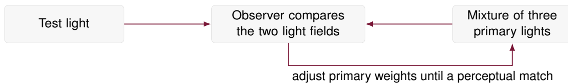
Figure 12.1. Conceptual color-matching experiment underlying trichromacy and Grassmann's laws.
