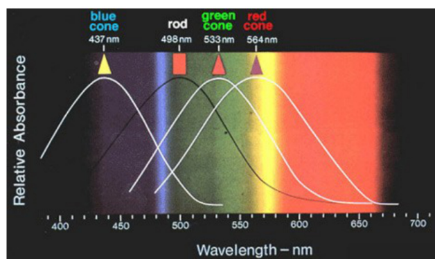
Figure 11.3. Lecture illustration of the three cone-sensitivity functions and their non-uniform representation.
