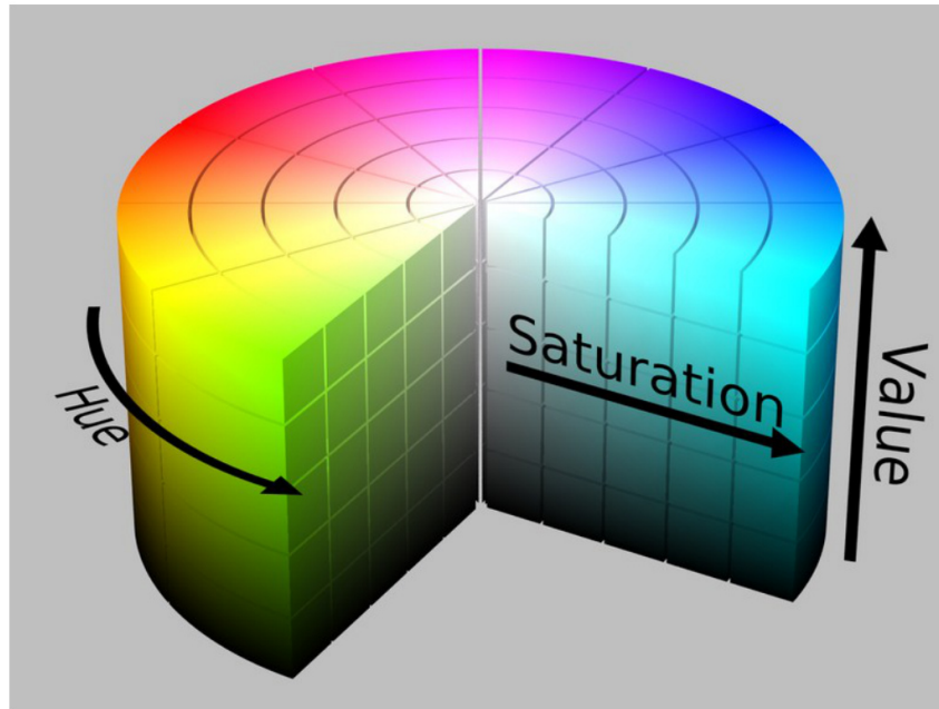
Figure 12.4. Geometric HSV representation shown in the lecture, emphasizing hue, saturation, and value as different axes of description.
