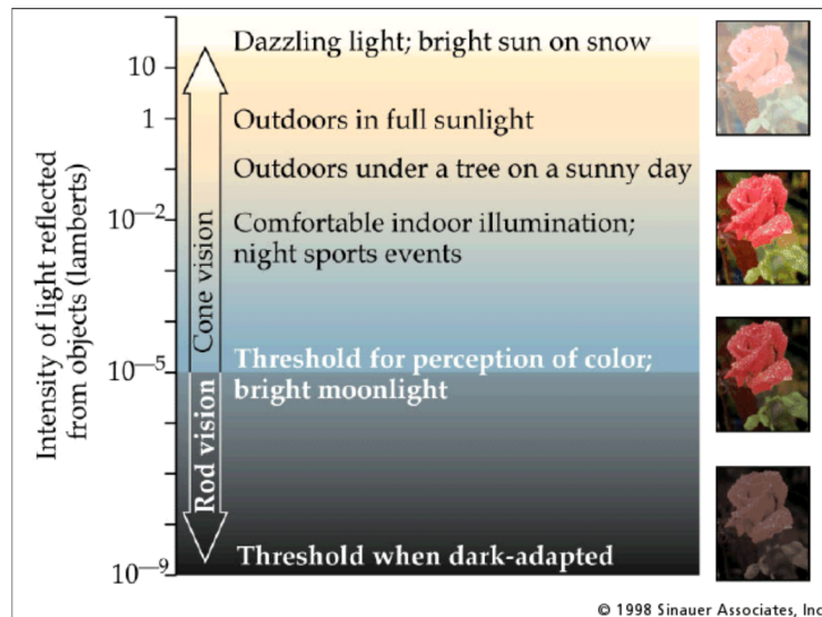
Figure 11.4. Source sensitivity regimes and light/dark adaptation thresholds. The chart is preserved rather than assigning invented numerical sensitivity curves.
