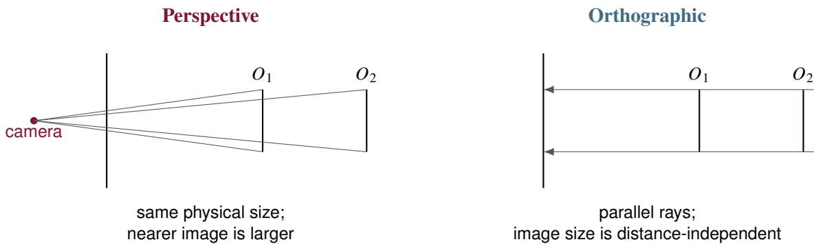
Figure 8.2. Conceptual contrast between perspective and orthographic projection.
