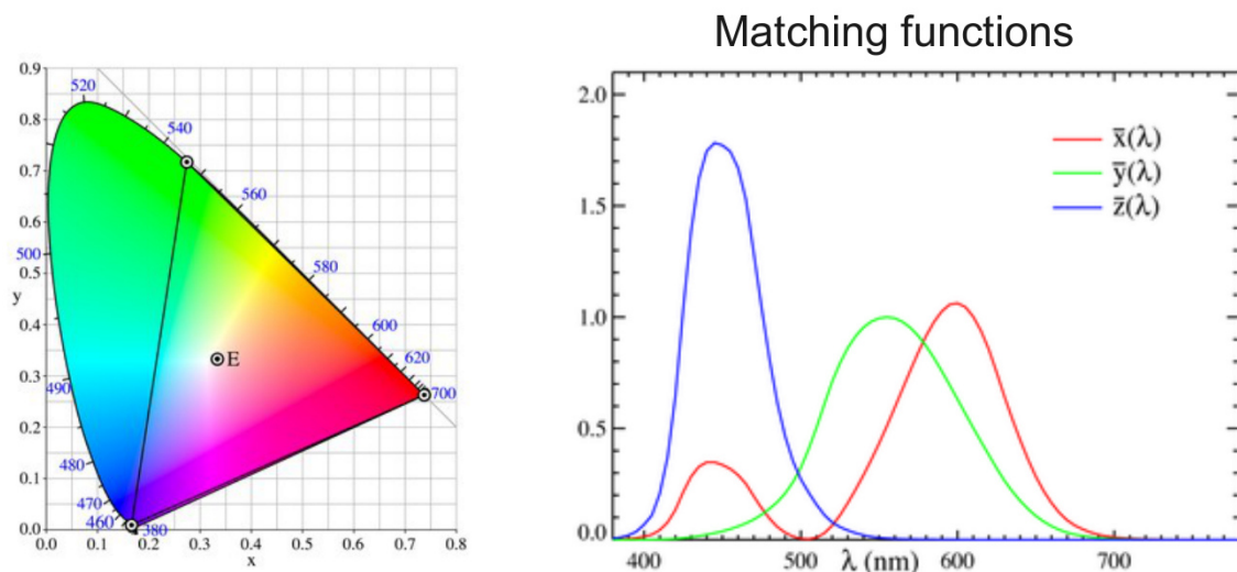
Figure 12.2. CIE XYZ material from the lecture: chromaticity visualization and the associated nonnegative matching functions.
