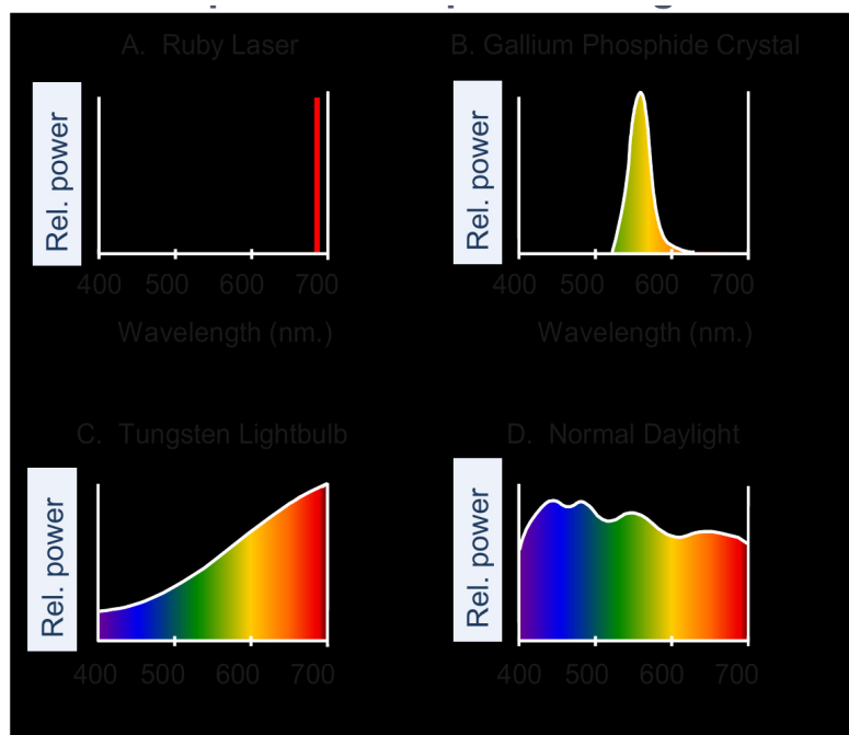
Figure 11.1. Examples from the lecture of qualitatively different source spectra, including narrow-band and broadband illumination.
