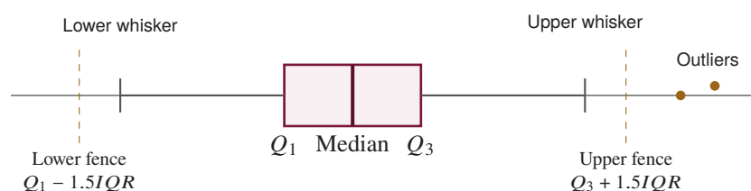
Figure 3.2: Schematic boxplot: the box spans the quartiles, the central line marks the median, and whiskers end at the most extreme observations within the fences.
