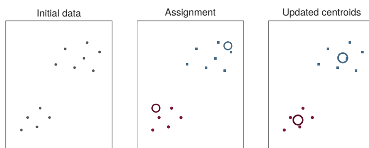
Figure 7.2: Schematic K-means assignment and centroid update. Filled points are observations; open circles are starting or updated centroids. Updated positions are the group means. Coordinates are illustrative.
