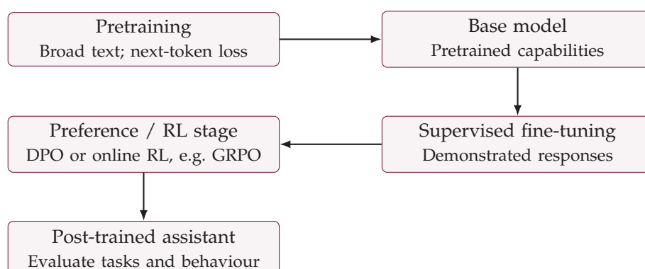
Figure 7.1: A typical combined workflow. Pretraining produces the base model; SFT and preference/RL training are subsequent stages. R1-Zero deliberately skips SFT, and other workflows can repeat stages.
