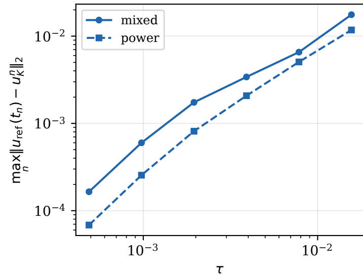
\gamma = 0.1, N = 8, K = 32
