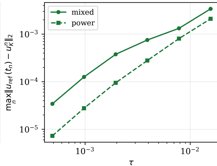
\gamma = 0.5, N = 8, K = 32
