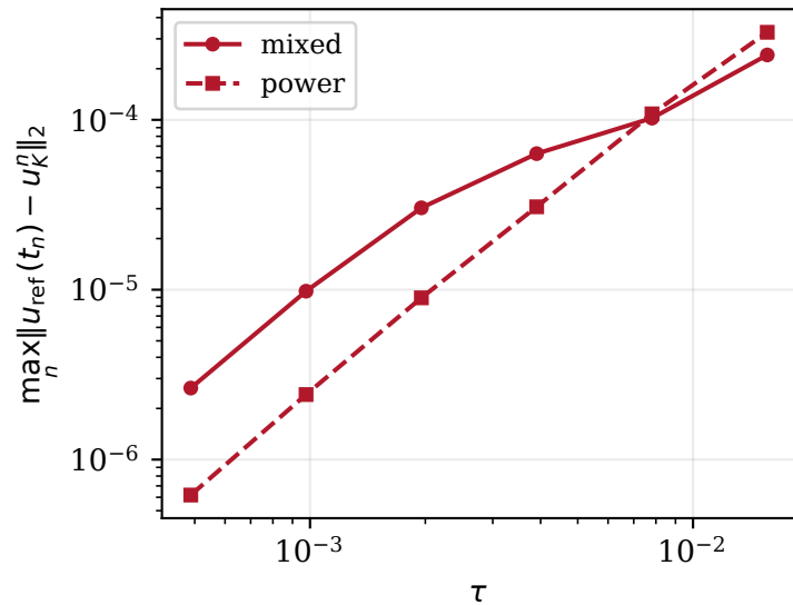
\gamma = 1, N = 8, K = 32
