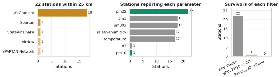
Figure 22. Stations near Dhaka by provider and by reported pollutant, and the number surviving each coverage filter. Generated from openaq_survey.json.
