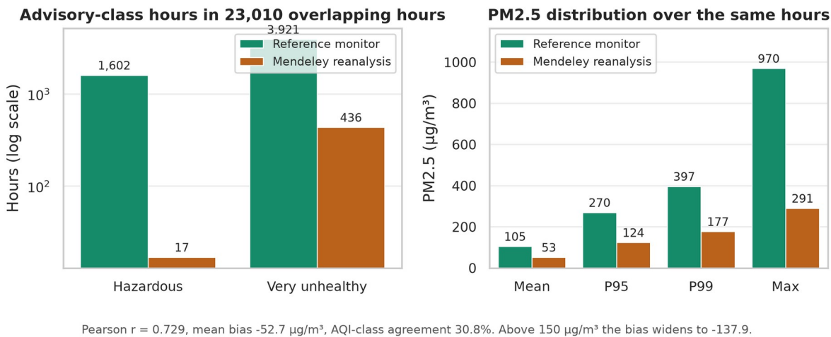
Figure 20. The reanalysis against the reference monitor over their overlapping period: advisory-class hours and the PM2.5 distribution. Generated from dhaka_ground_truth.json.
