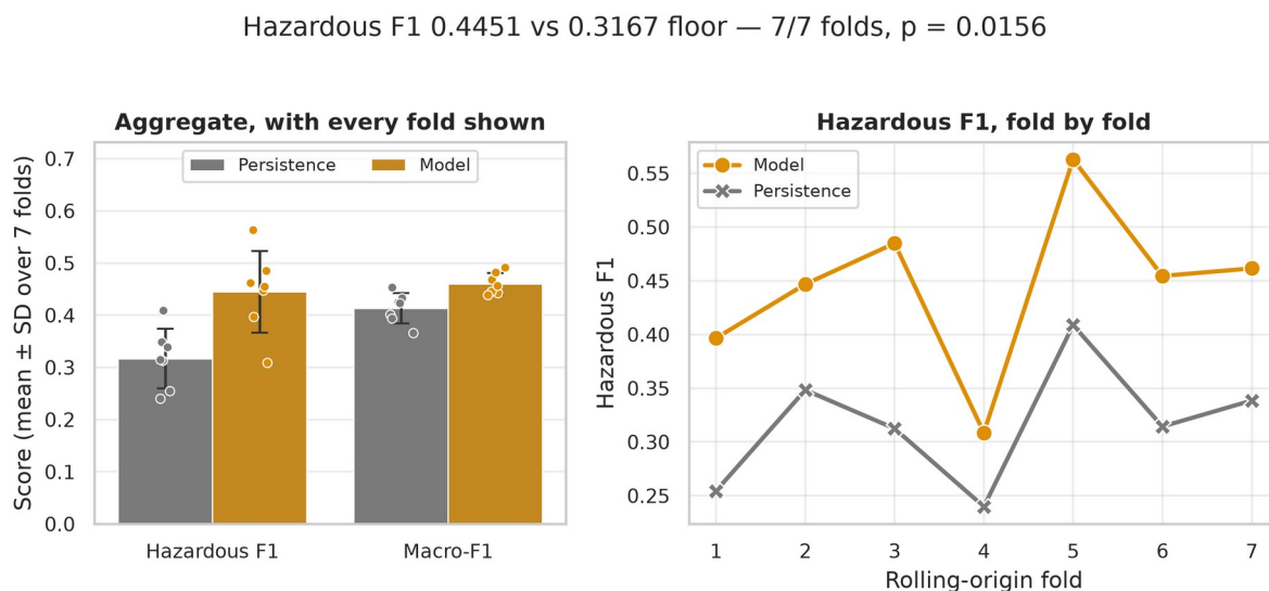
Figure 21. Hazardous-class and aggregate performance against the persistence floor across seven rolling-origin folds, with every fold shown. Generated from dhaka_pm25_model_h6.json.
