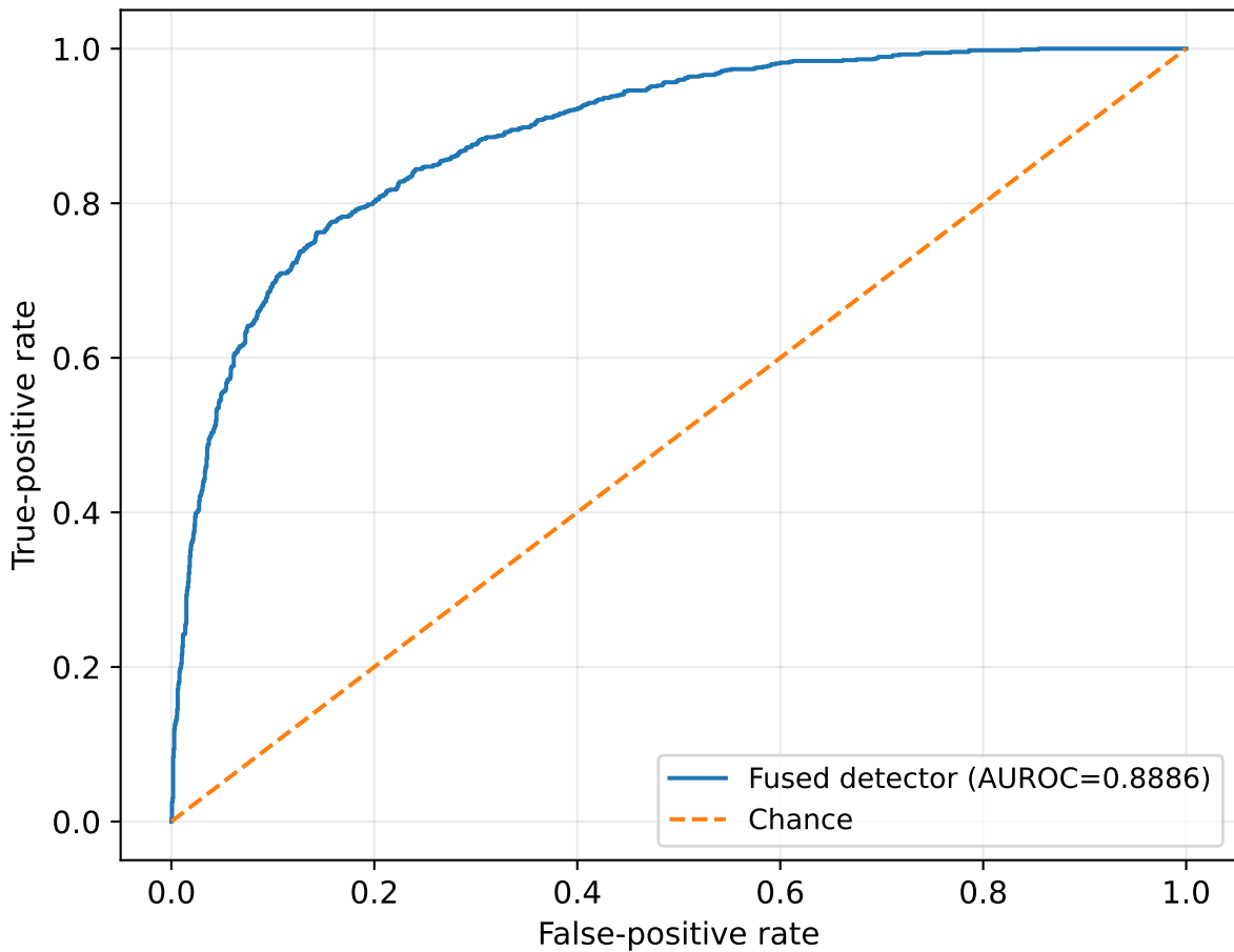
Official RAGTruth test ROC
