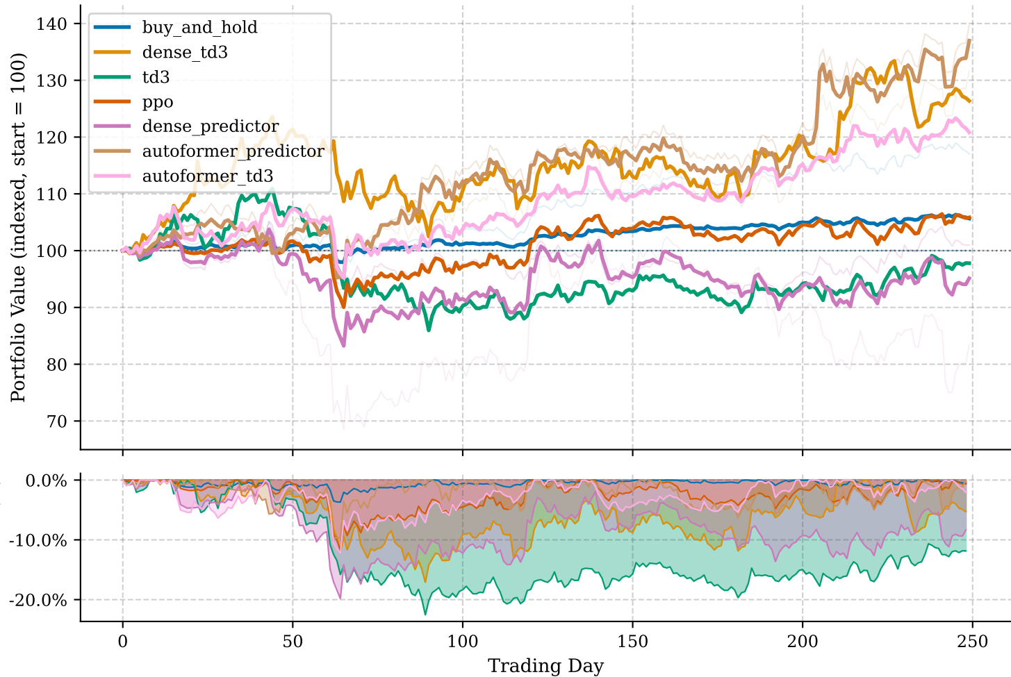
Portfolio Performance — sp100
