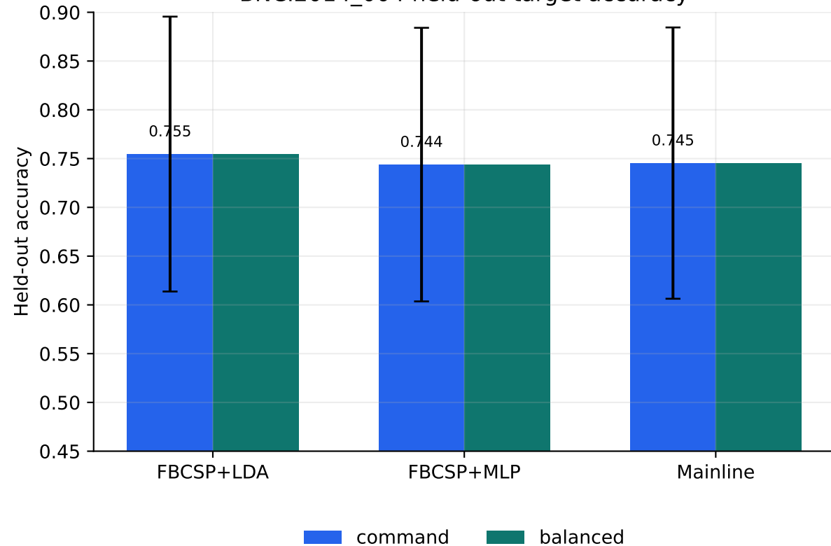
BNCI2014_004 held-out target accuracy
