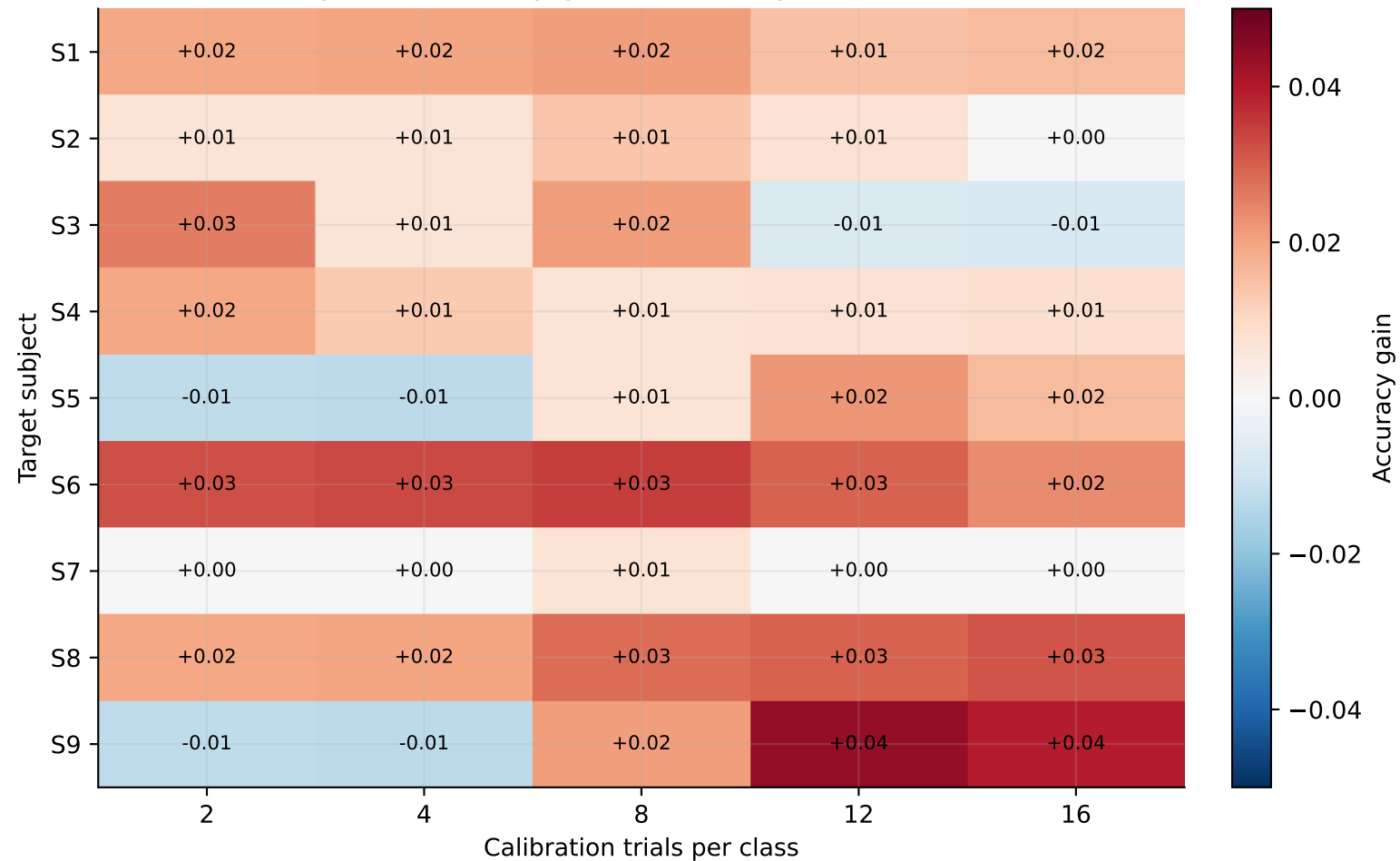
Experience-library gain vs before personalization
