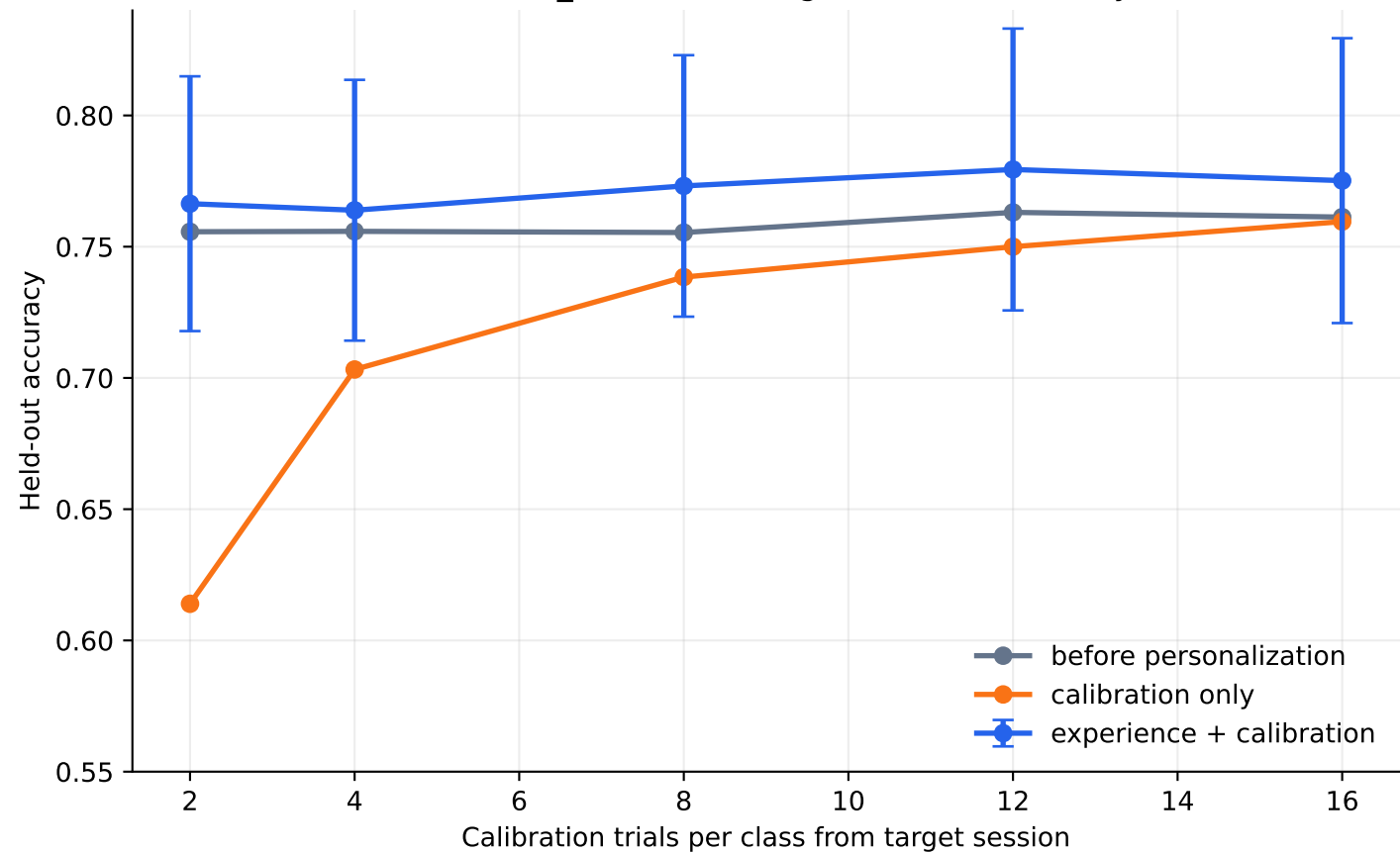
BNCI2014_004: mean target-session accuracy
