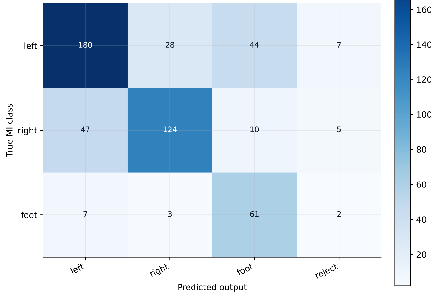
Photonic-scan confusion
