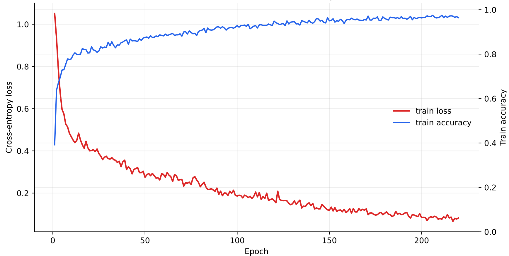
Mainline shared encoder training
