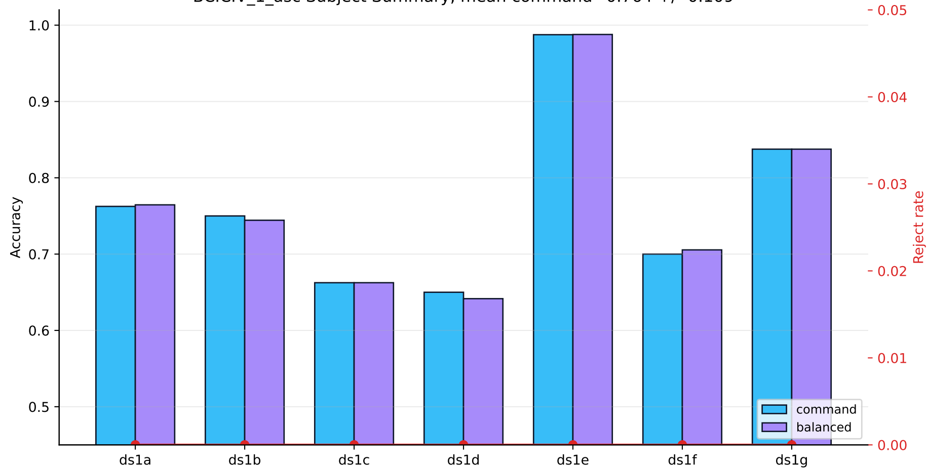
BCICIV_1_asc Subject Summary, mean command=0.764 +/- 0.109
