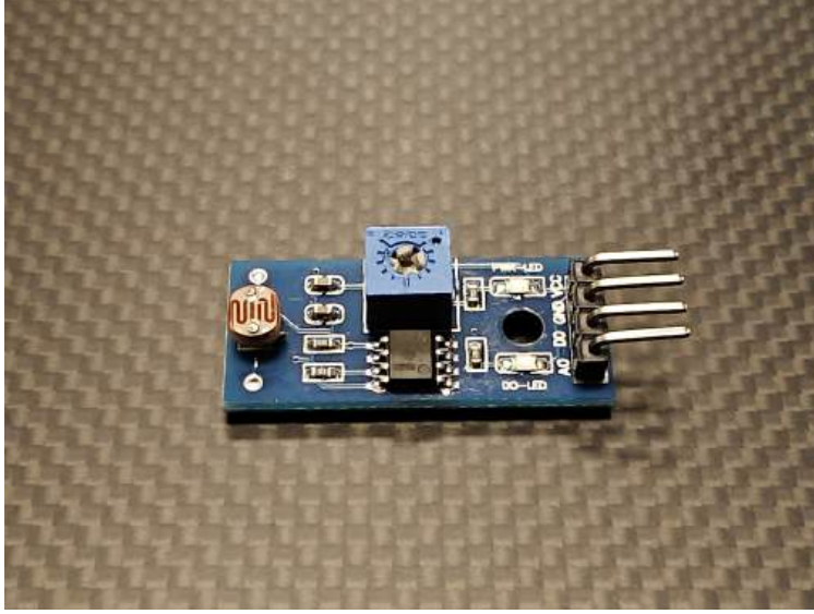
Figure 4: Analog light sensor used to measure light intensity in the light-source NH-ES experiment.
