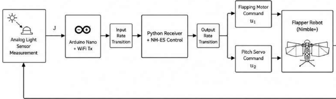
Figure 5: Simplified discrete-time control and communication architecture for the light-source-seeking NH-ES experiment. The analog light sensor measurement is read by the Arduino Nano and transmitted wirelessly to the Python receiver, where the NH-ES control law is implemented. The first rate-transition block represents the transition from the sensor/Arduino transmission rate to the Python control update rate, while the second rate-transition block represents the transition from the Python command update rate to the flapper-board actuation rate.
